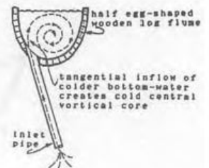
Fig. 12.10b Section thro' flume
