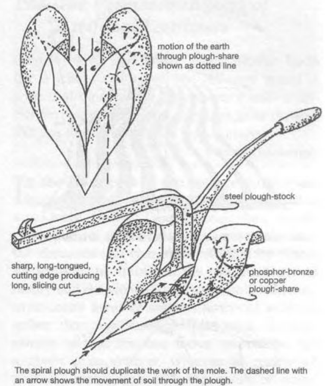
Fig. 19.5 & 6 "The Bio-Plough", 1948
