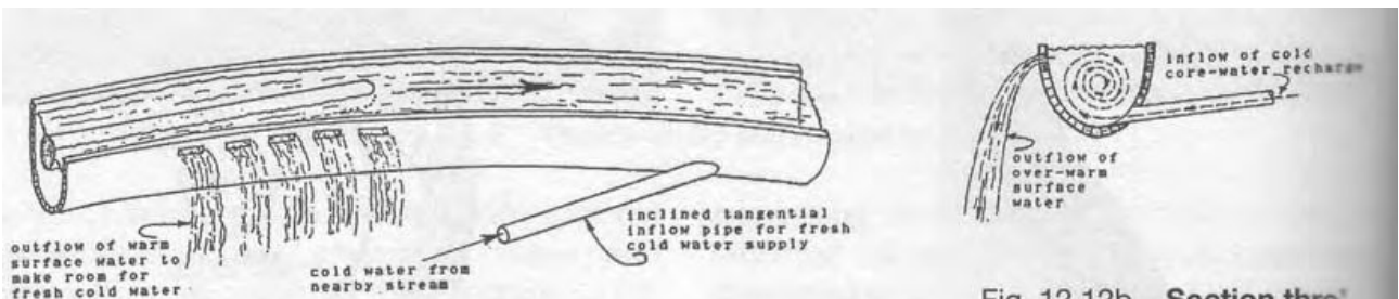
Fig. 12.12a Detail of warm/cold water exchange
